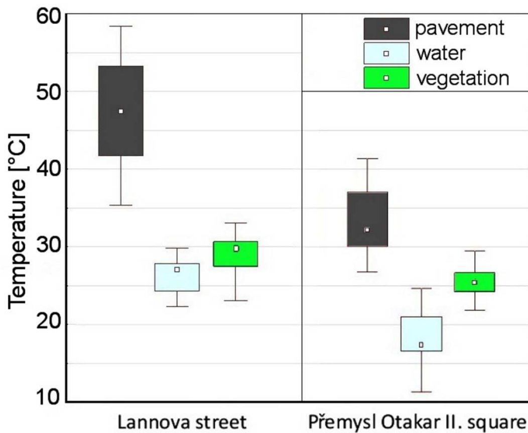
Figure 9: Comparison of ST of a green structure, a blue structure and pavement
