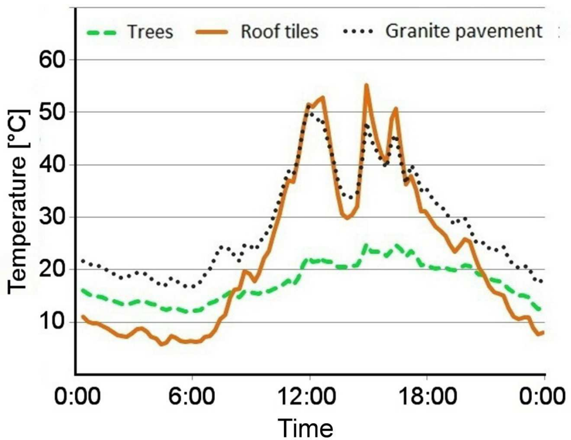
Figure 3: Comparison of ST of trees, roof tiles and granite pavement
