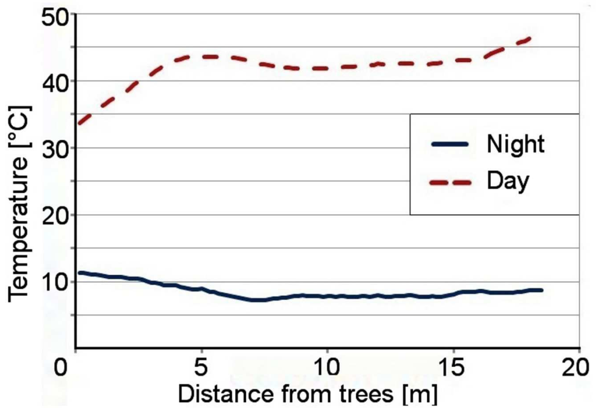
Figure 4: The buffering effect of tree canopies on the roof tiles ST
