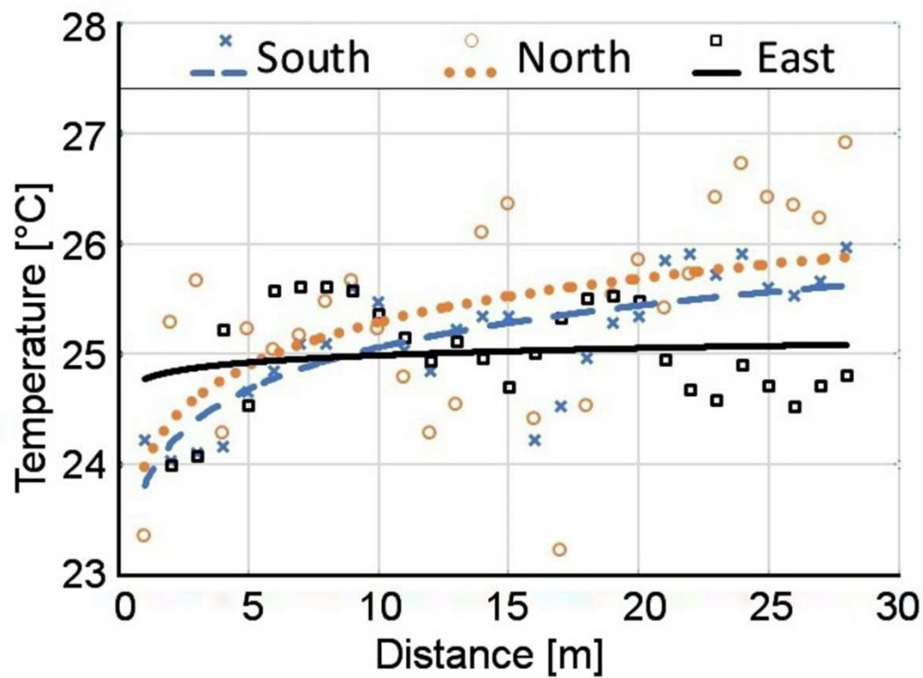
Figure 8: The cooling effect of the fountain depending on directions
