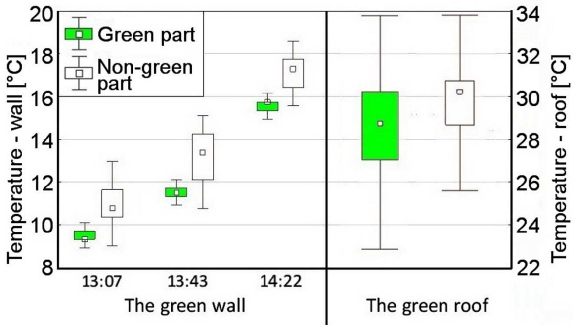
Figure 6: Thermal comparison of the green and non-green parts of the roof and the wall
